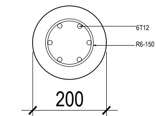
COLUMN C1 DETAIL
