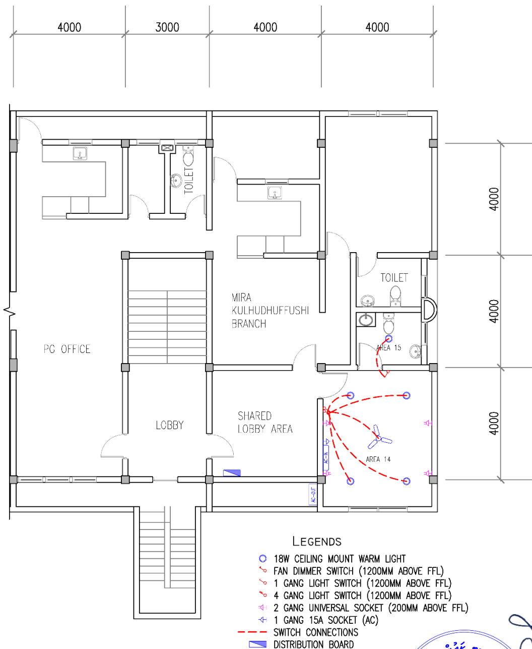
THIRD FLOOR ELECTRICAL PLAN
