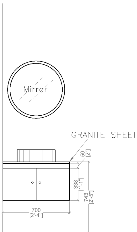
WASH BASIN
