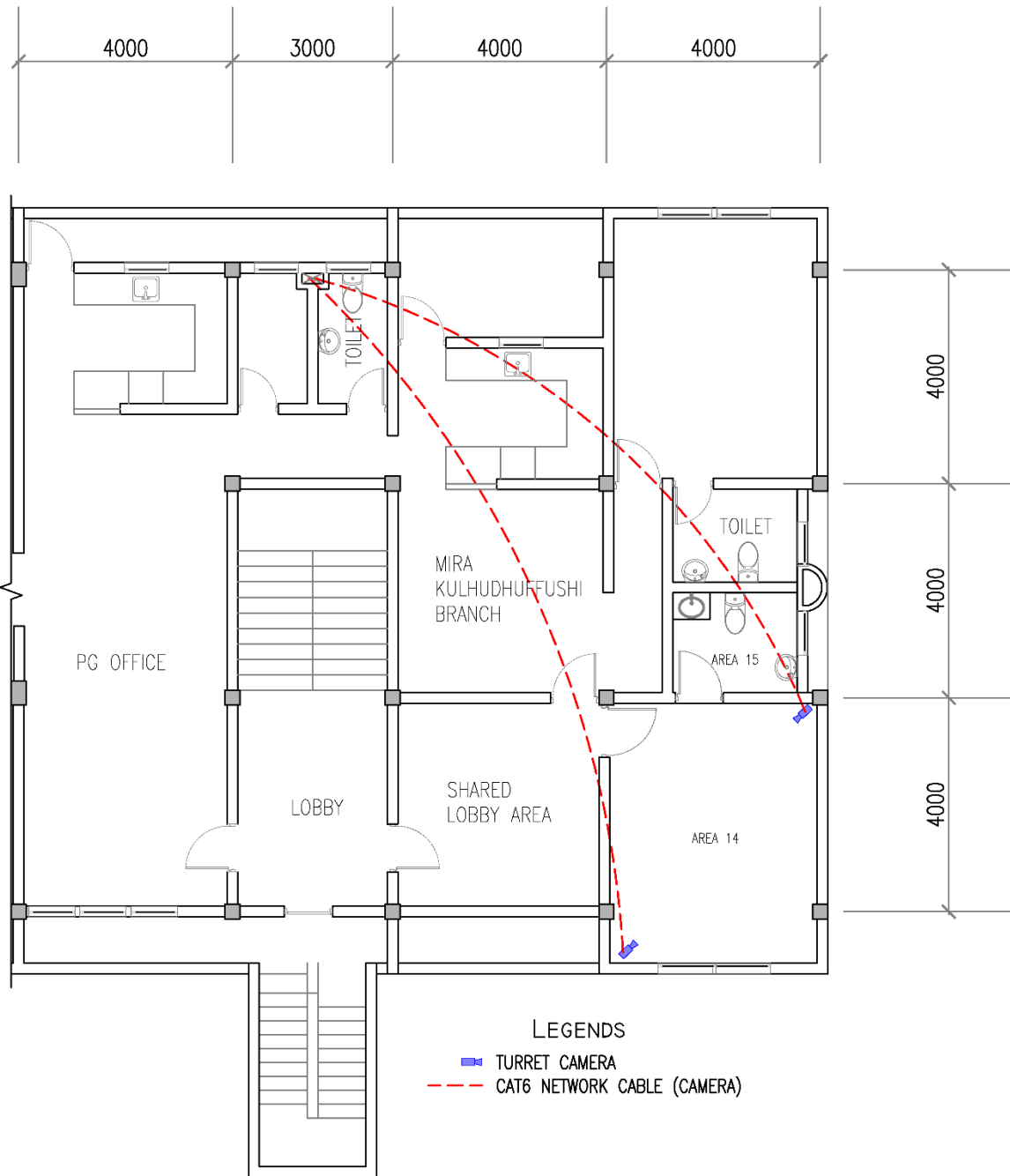
THIRD FLOOR CCTV LAYOUT
