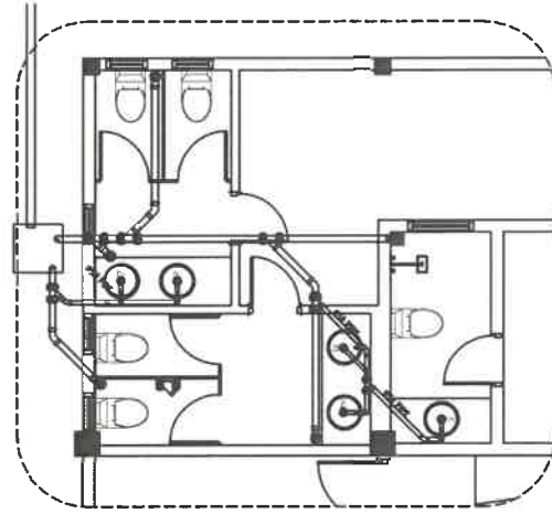
DETAIL-1 WASTE WATER DISPOSAL LAYOUT SCALE 1/50
