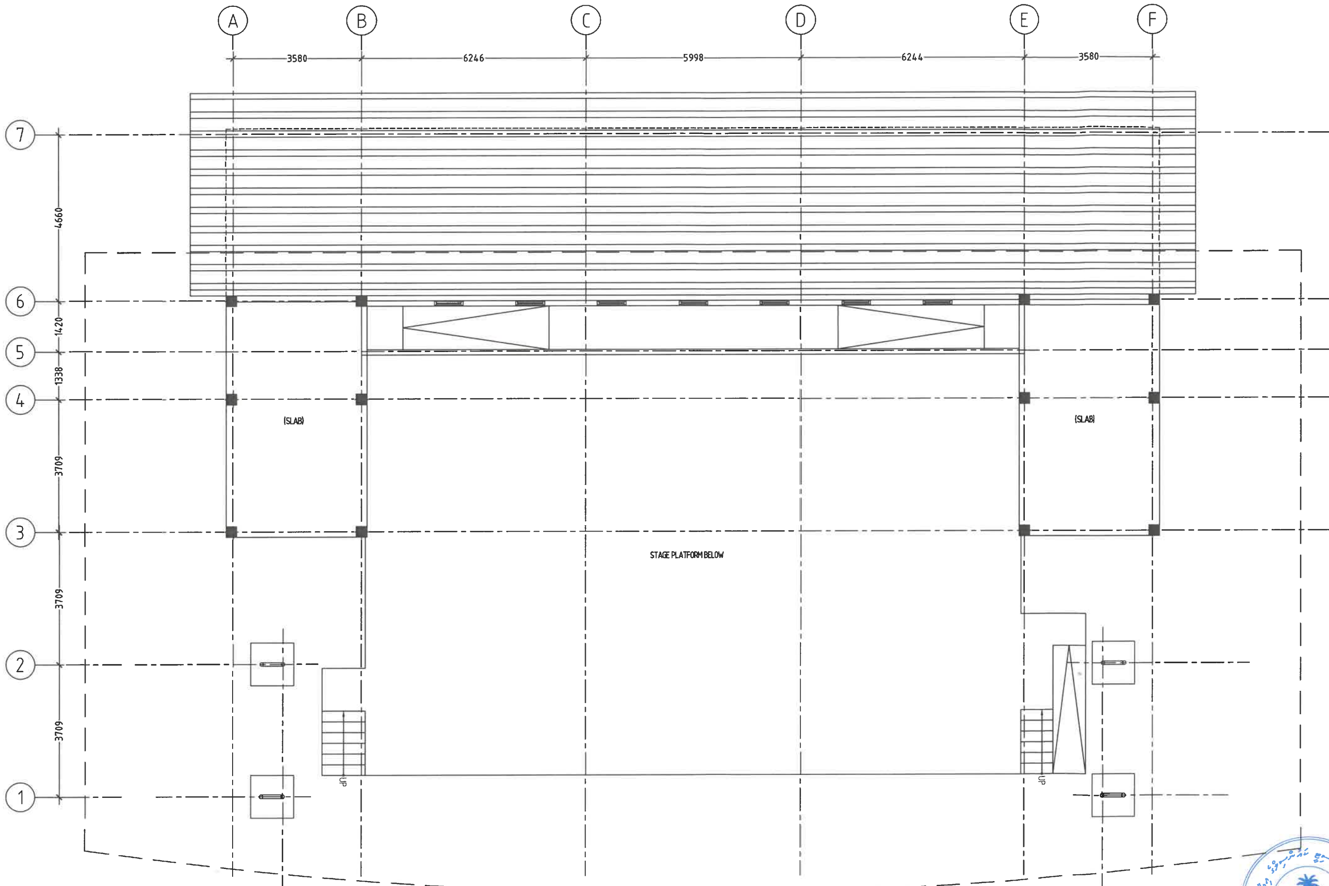
FLOOR PLAN-2 SCALE 1:100
