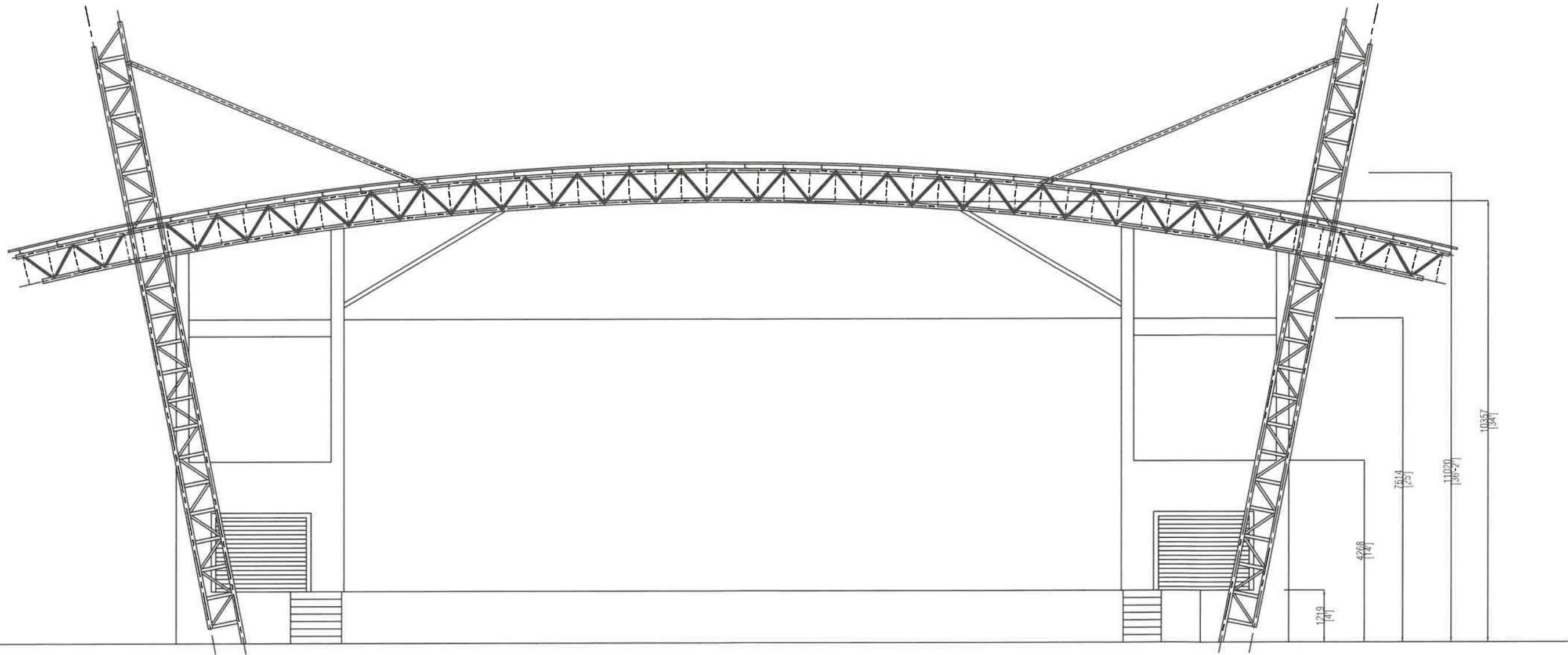
FRONT ELEVATION SCALE 1:100
