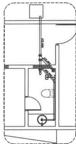
DETAIL-2 WASTE WATER DISPOSAL LAYOUT SCALE 1/50
