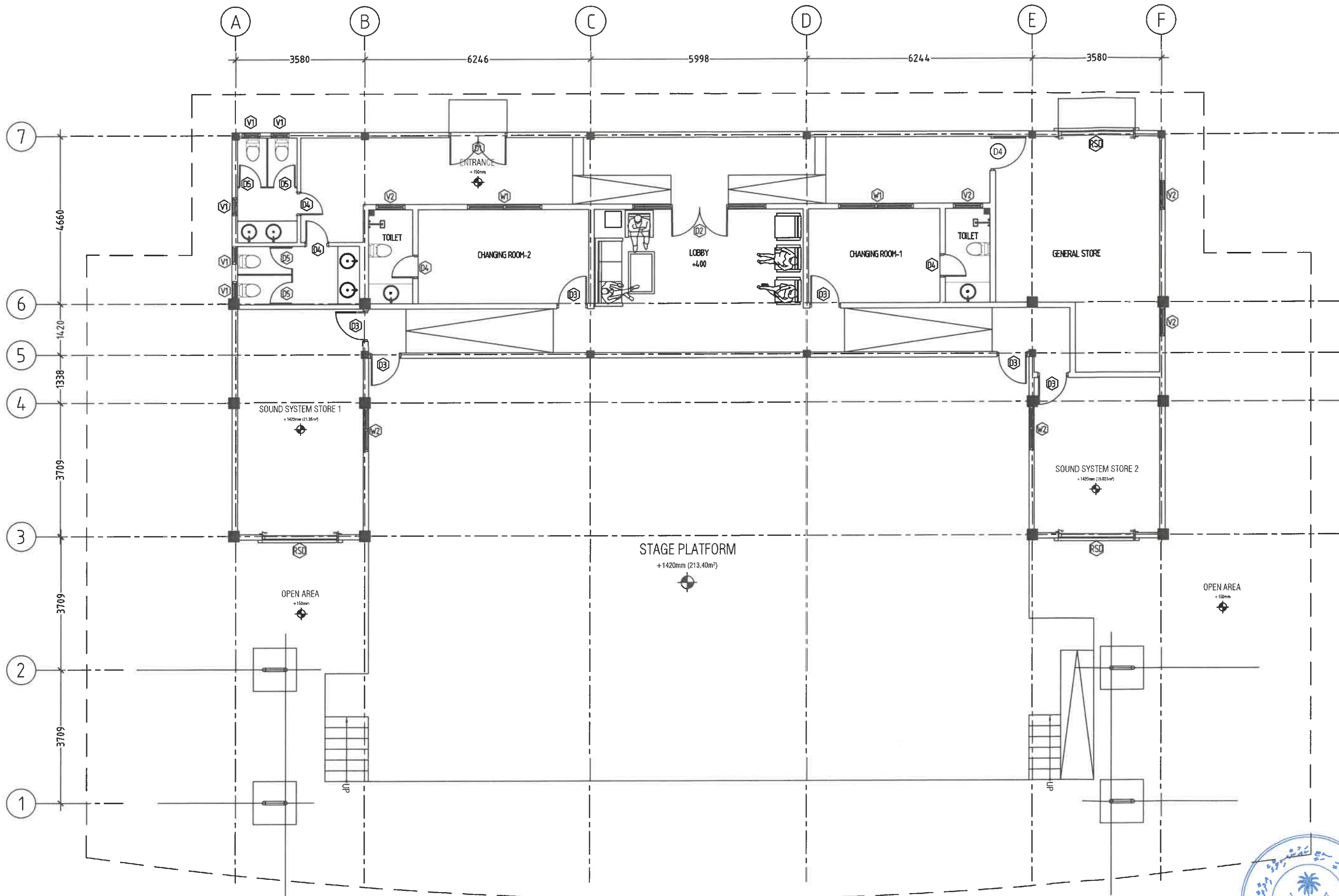
FLOOR PLAN-1 SCALE 1:100
