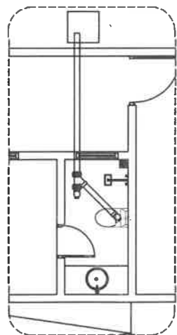
DETAIL-2 SEWAGE DISPOSAL LAYOUT SCALE 1/50
