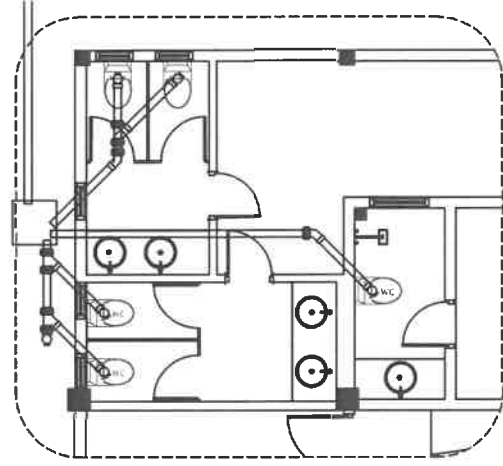
DETAIL-1 SEWAGE DISPOSAL LAYOUT SCALE 1/50
