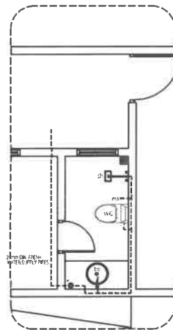
DETAIL-1 FRESH WATER SUPPLY LAYOUT SCALE 1/50
