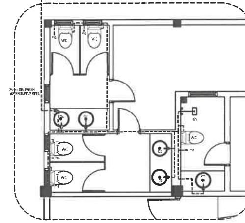
DETAIL-1 FRESH WATER SUPPLY LAYOUT SCALE 1/50
