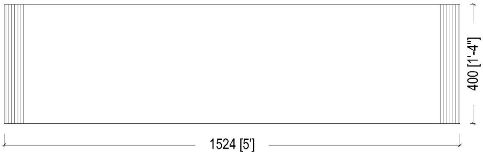
TOP VIEW
